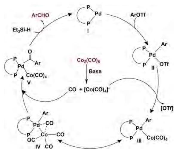
Scheme 3. Mechanistic Proposal.
