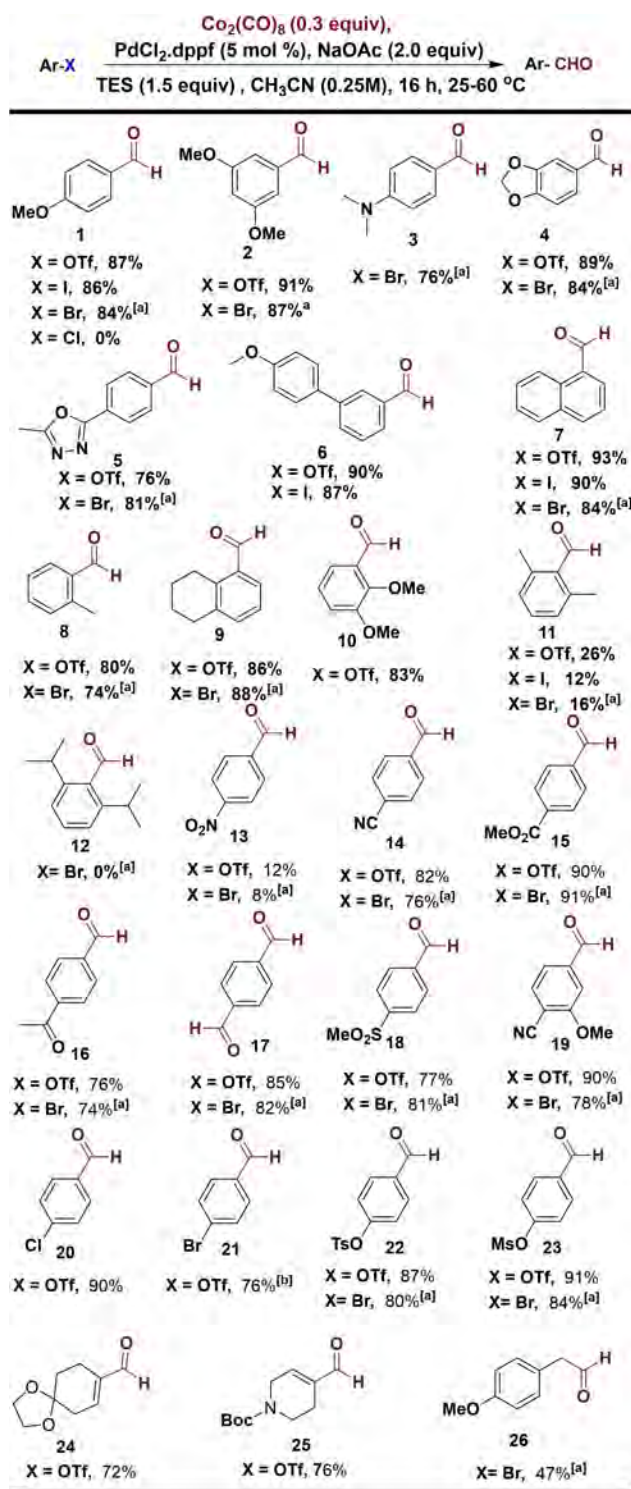
Scheme 1. Reductive Carbonylation of Ar-X/OTf. Reaction condition: Ar-X/OTf (1 mmol), catalyst, base, solvent (0.25 M). Isolated yields reported. [a] At 60 °C, 16 h. [b] 16% of dicarboxaldehyde.
