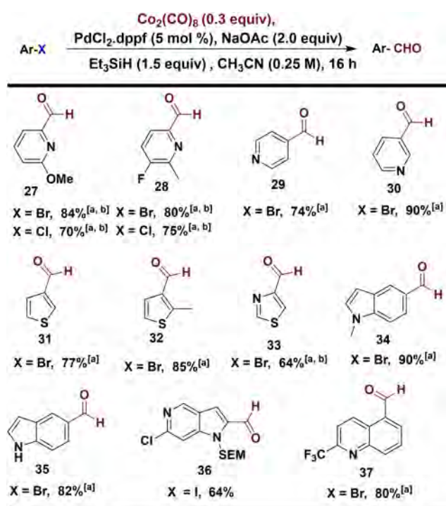
Scheme 2. Reductive carbonylation of heteroaromatic halides. Reaction condition: Ar-X (1.0 mmol), catalyst, base, solvent (0.25 M). [a] At 60 °C, 16 h. [b] With 1.0 equiv. of TBAB.
